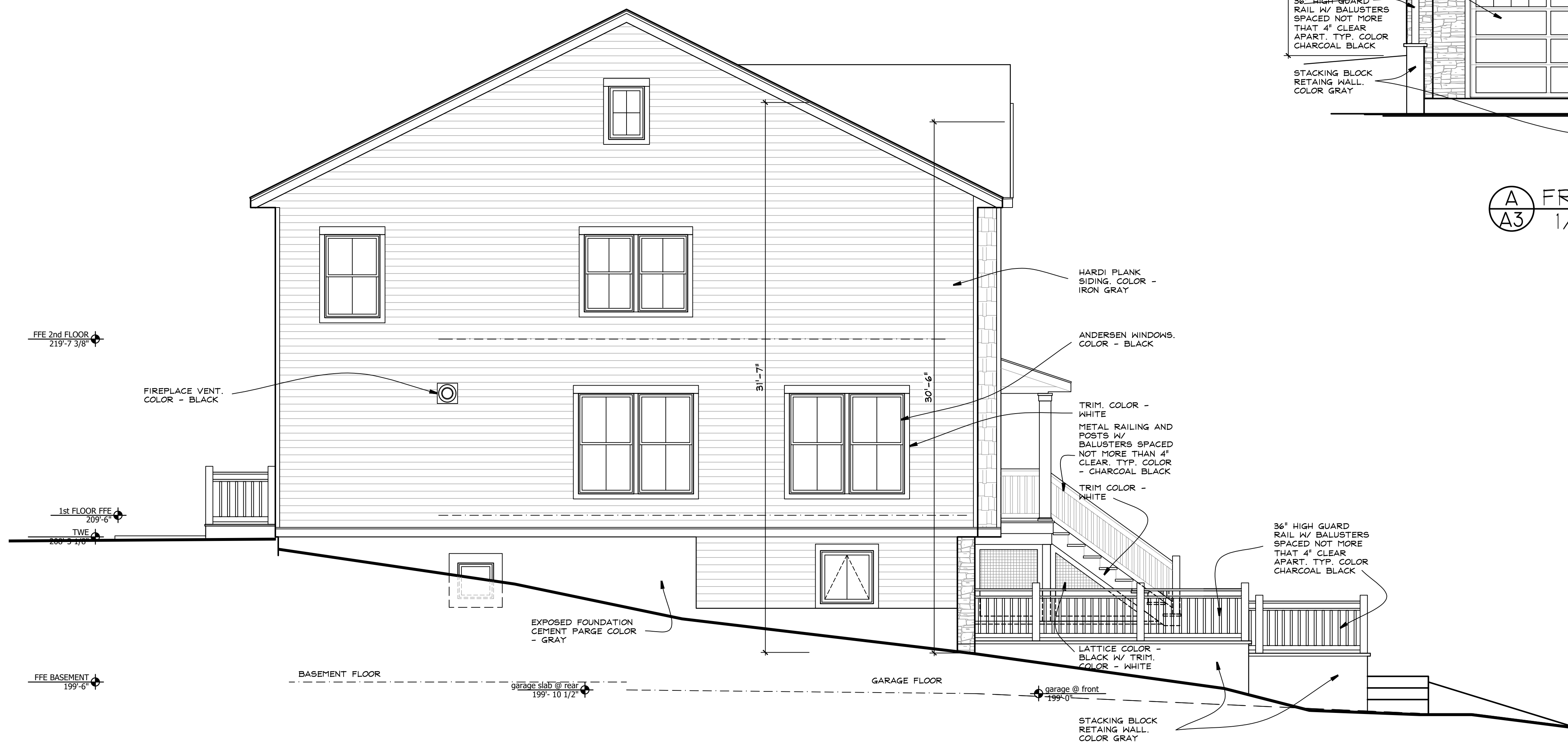
B SOUTH SIDE ELEVATION A3 1/4" = 1 FOOT
