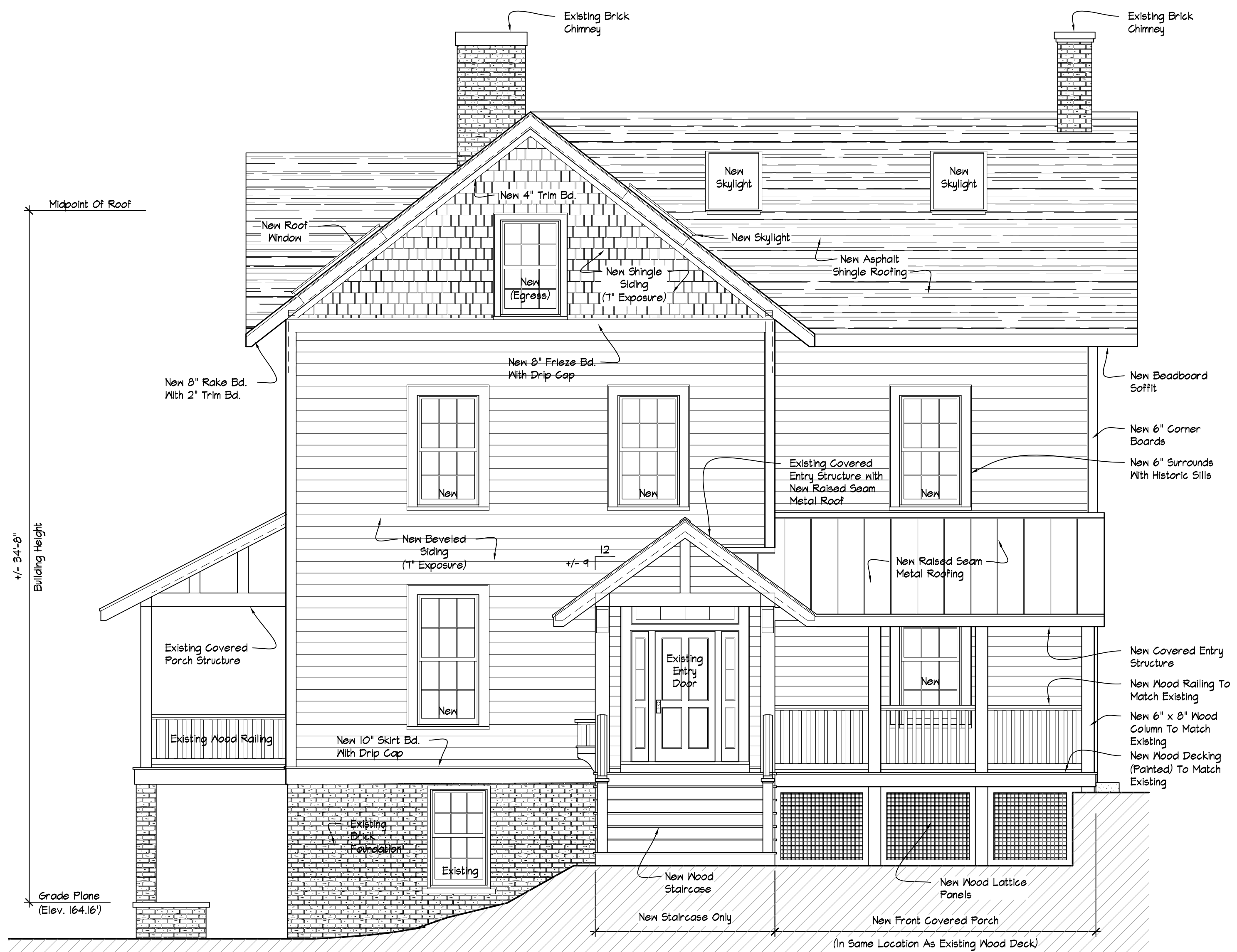
1 FRONT ELEVATION SCALE: 1/4" = 1'-0" NORTH FAÇADE
