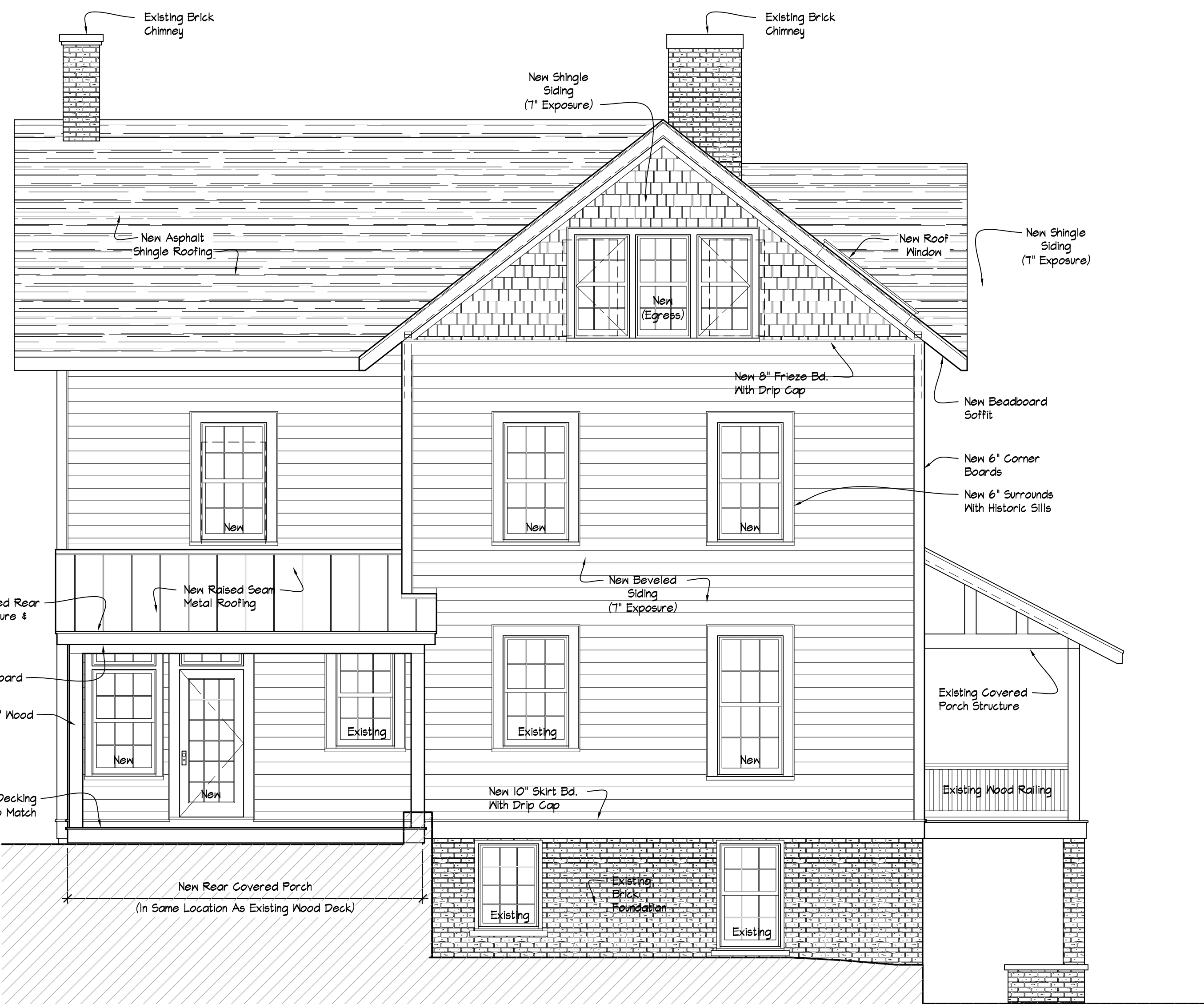
1 REAR ELEVATION SCALE: 1/4" = 1'-0" SOUTH FAÇADE
