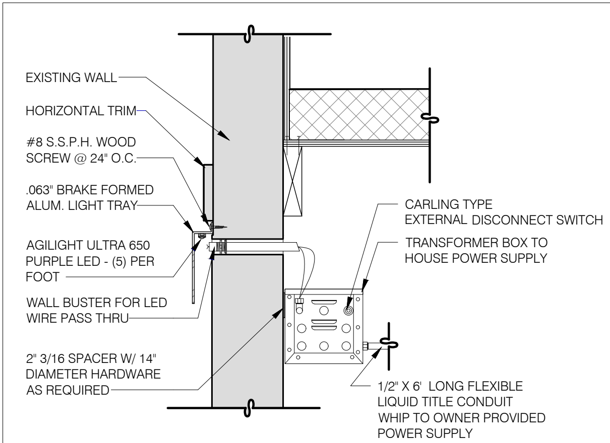
LED WALL WASHER DETAIL N.T.S. E
