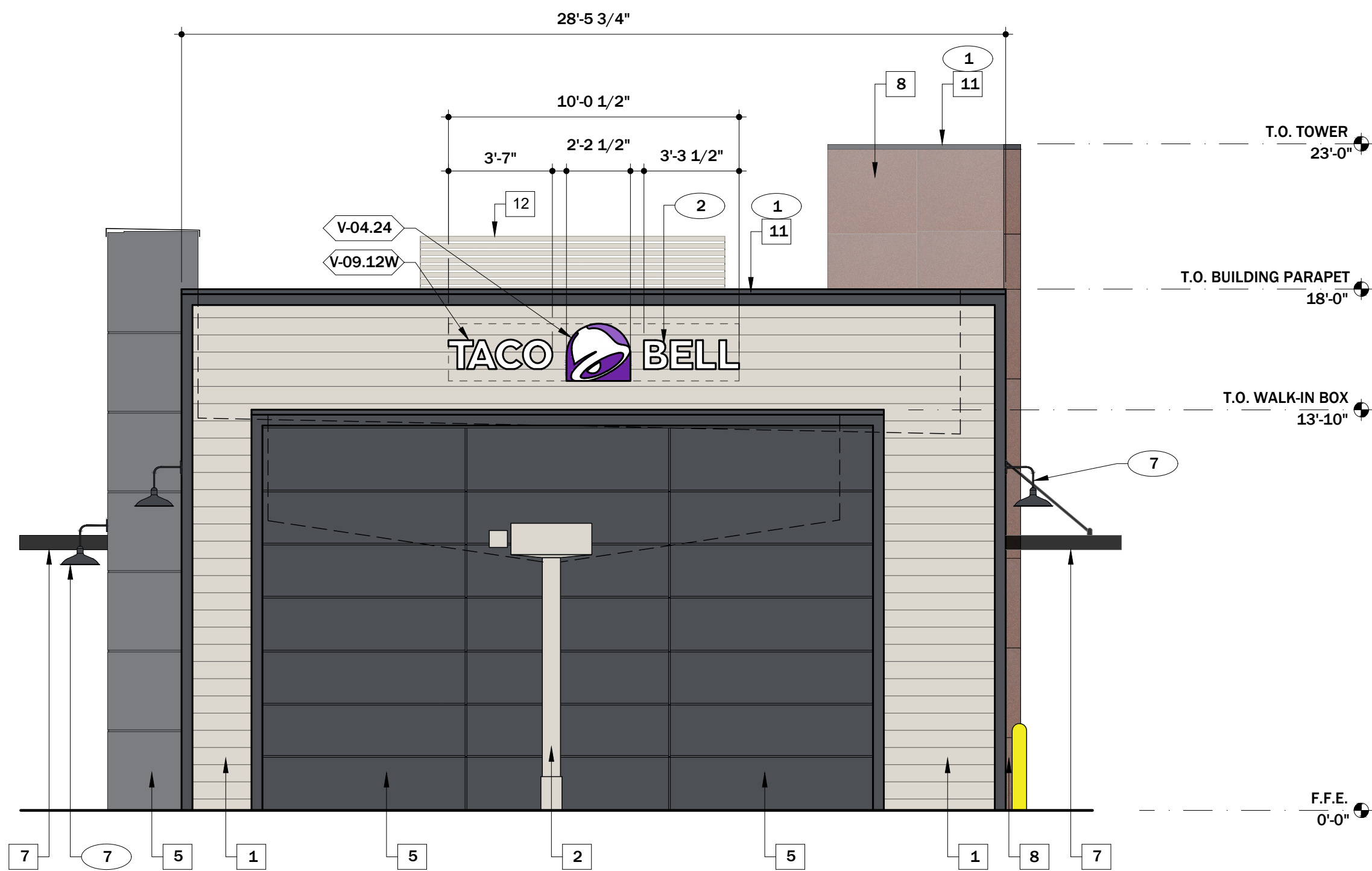
WEST ELEVATION 1/4" = 1'-0" A
