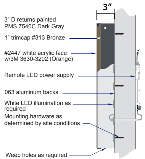
ORANGE CUP ICON & LETTER "D" SECTION VIEW
