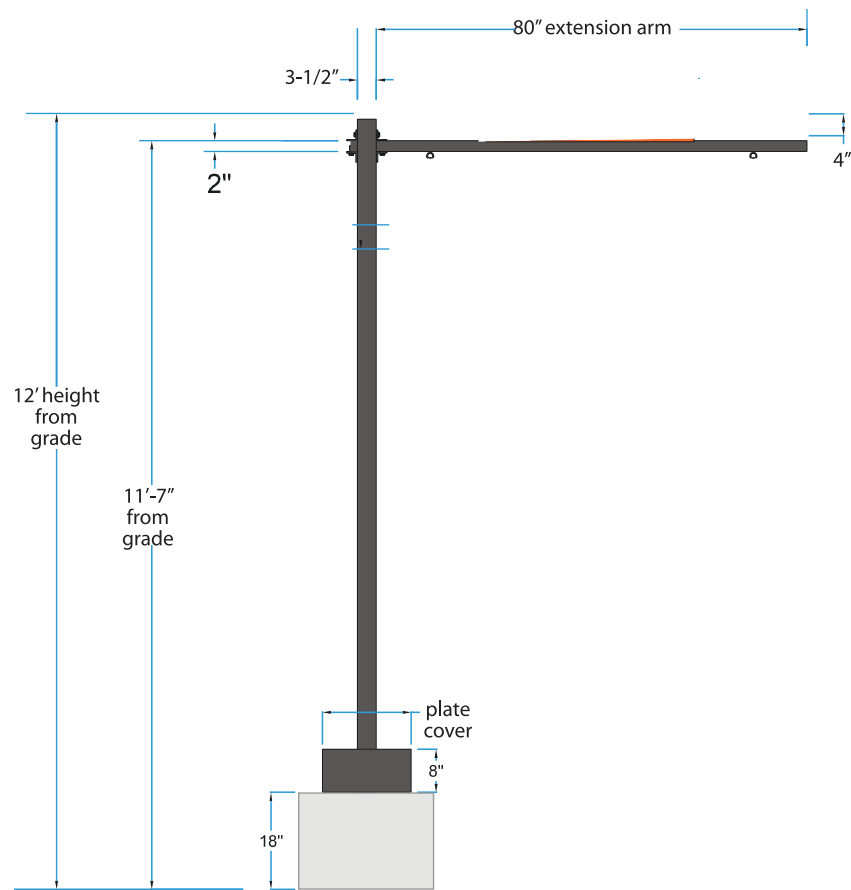
SINGLE ARM VEHICLE HEIGHT DETECTOR
