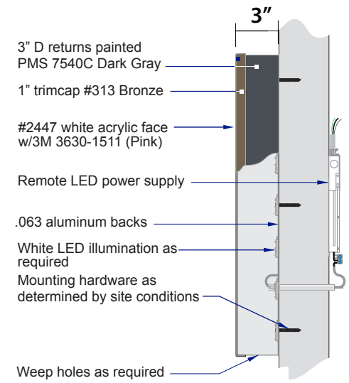
MAGENTA APOSTROPHE SECTION VIEW
